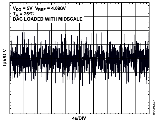
Figure 30. 0.1 Hz to 10 Hz Output Noise Plot
