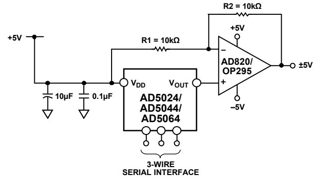
Figure 53. Bipolar Operation
