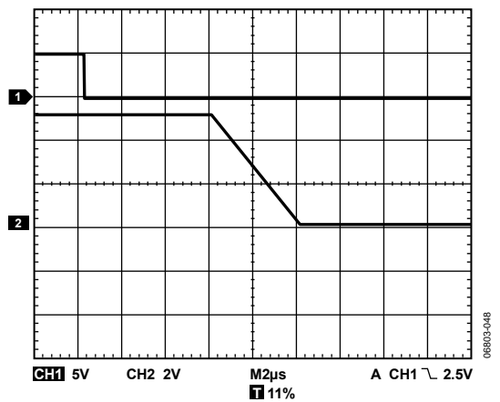
Figure 33. Hardware \overline{CLR}
